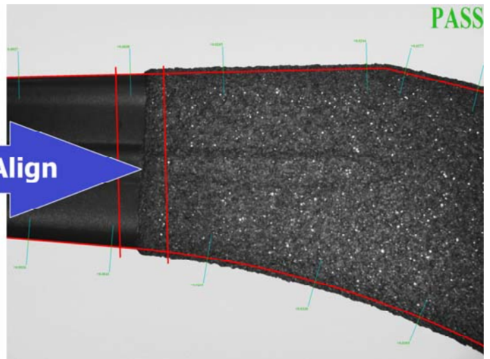
The Auto-Align tool automatically aligns the CAD data to the part, almost instantly, along an arbitrary number of user-specified datums
